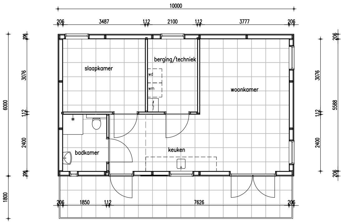
Beganeground
